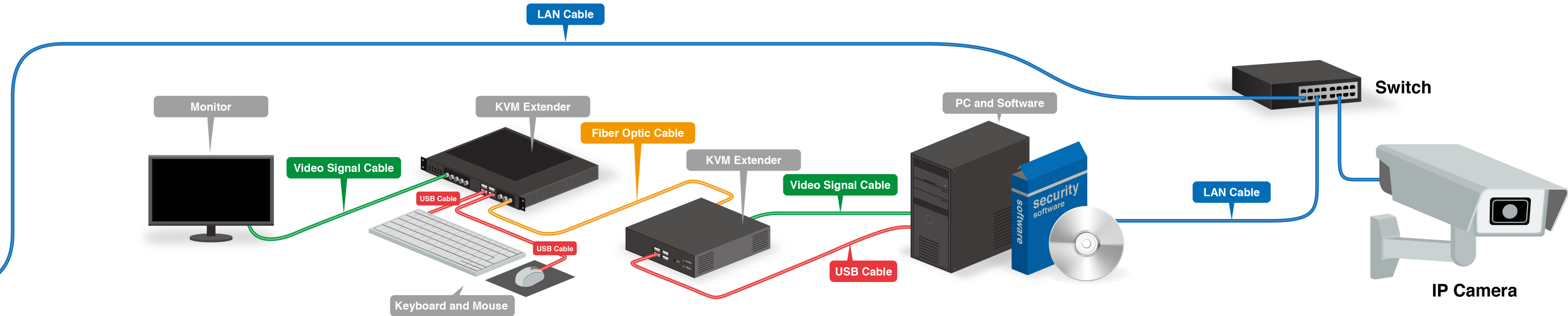
Conventional Installation
